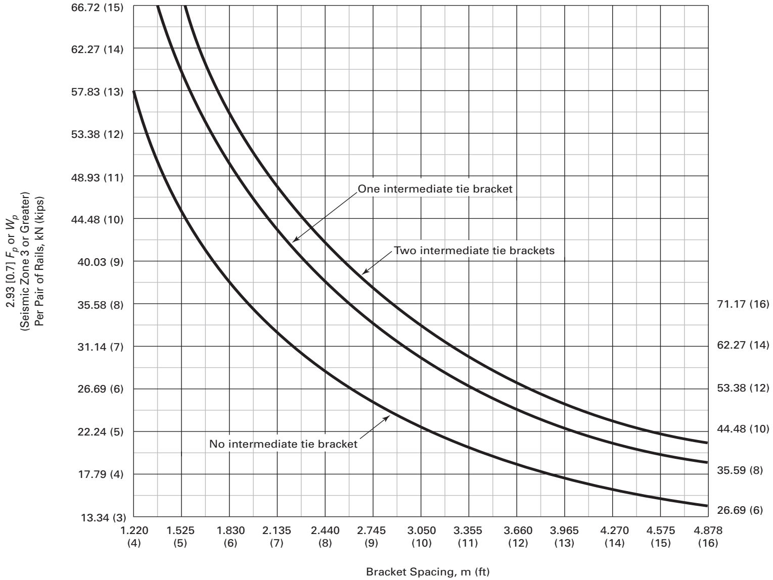
Fig. 8.4.8.2-1 12 kg/m (8 lb/ft) Guide-Rail Bracket Spacing
