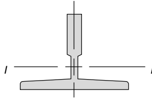
Fig. 2.23.4.1-2 Minimum Moment of Inertia About x-x Axis for a Single Guide Rail With Its Reinforcement
