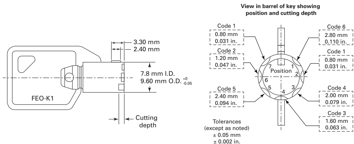
Fig. 2.27.8 FEO-K1 Key
