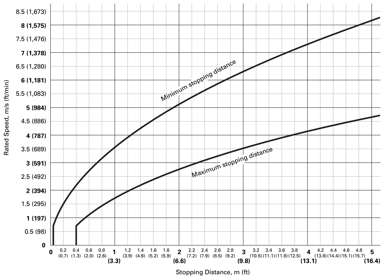
Fig. 8.2.6 Stopping Distances for Type B Car and Counterweight Safeties
