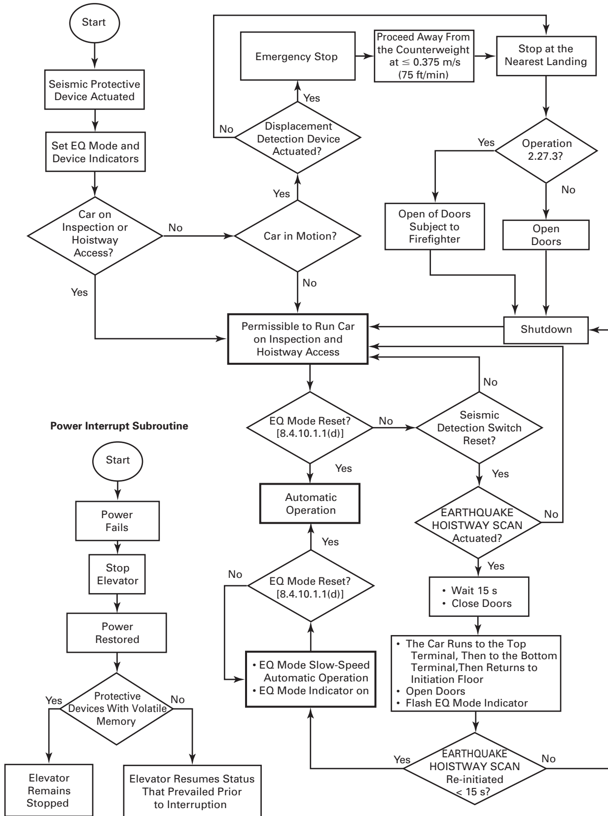
Fig. 8.4.10.1.3 Earthquake Emergency Operation Diagrammatic Representation
